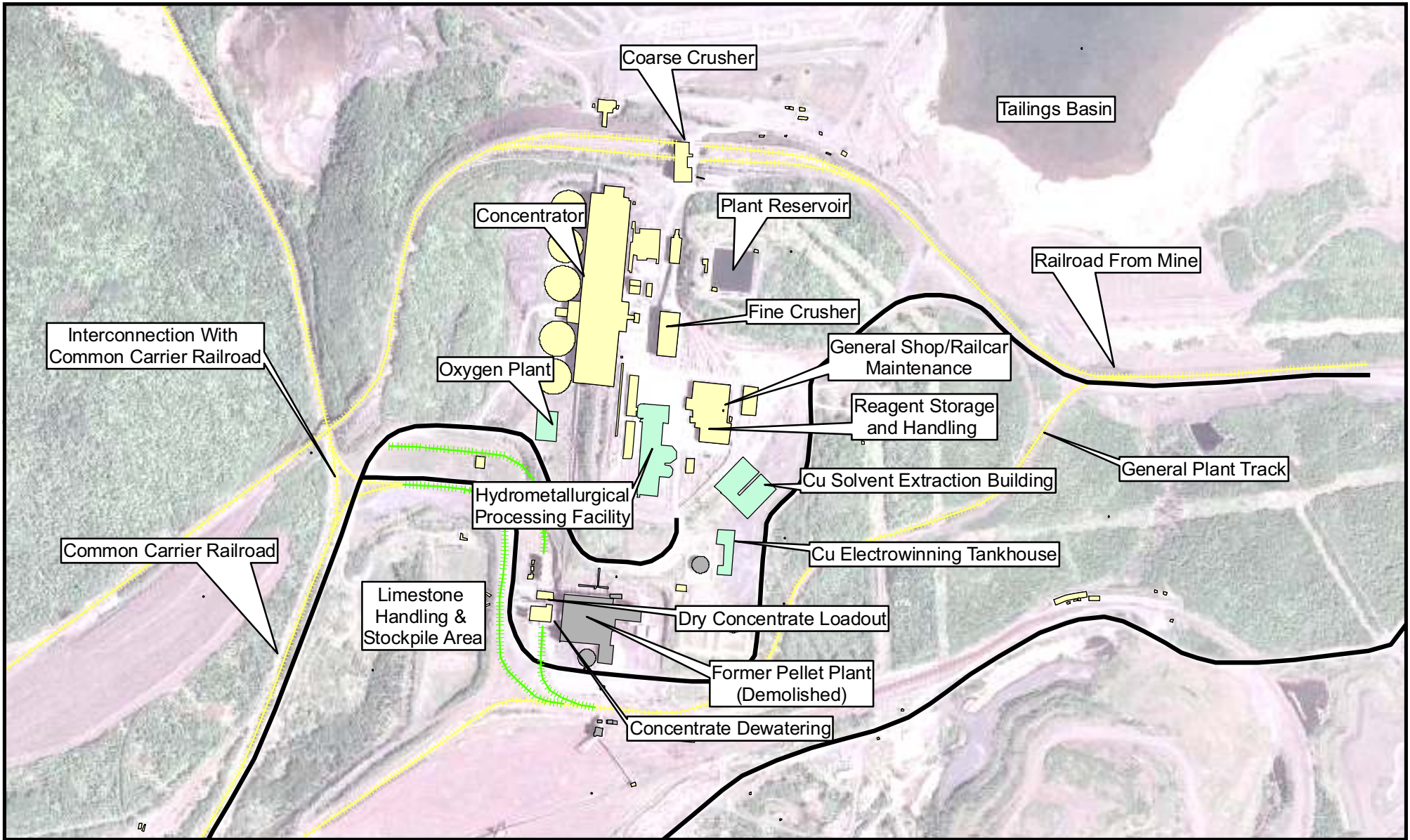
Figure 3.1-17a Processing Plant (All Actions)
